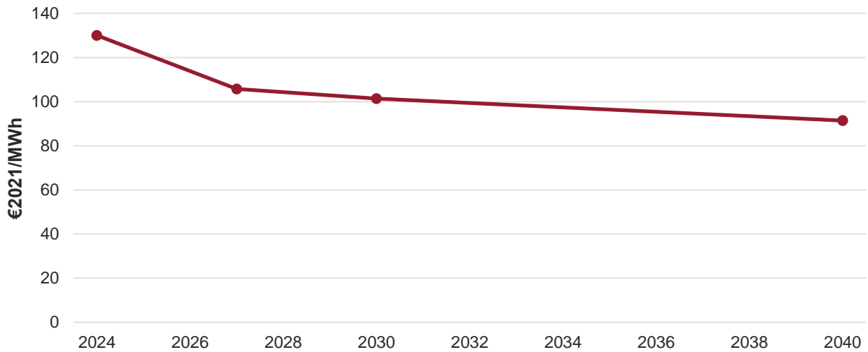
Figure 17 Reference scenario: Average wholesale electricity prices
